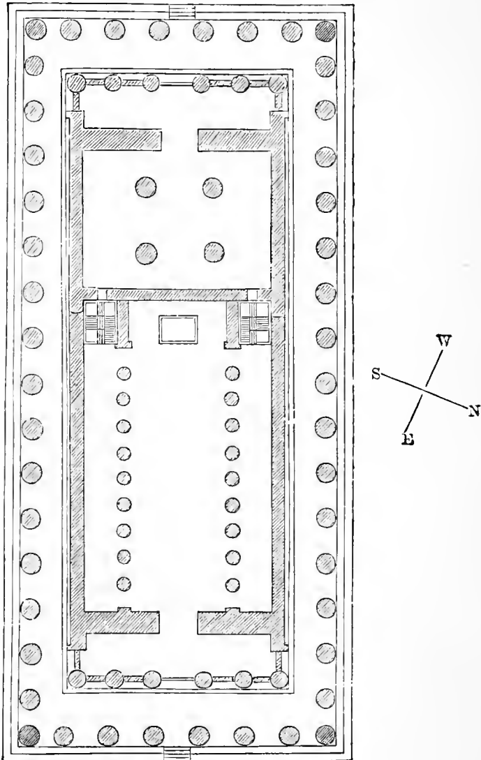
FIG. 53.—PLAN OF THE PARTHENON AT ATHENS.
